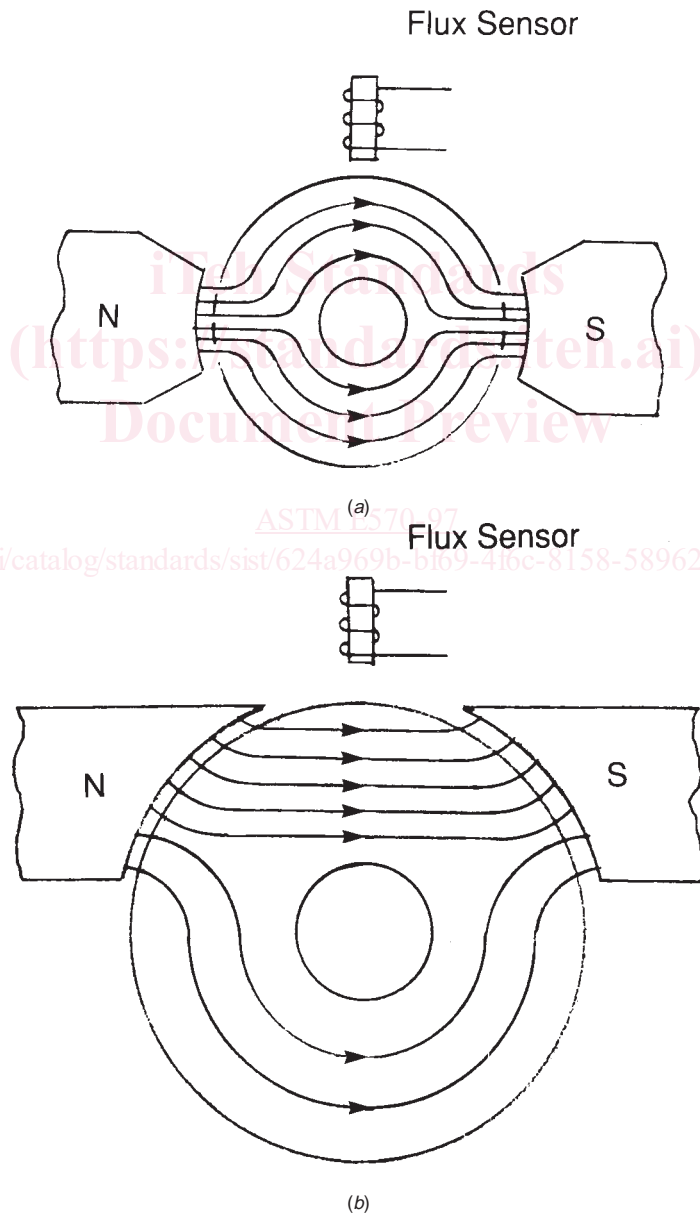
FIG. 1 Transverse Magnetization
