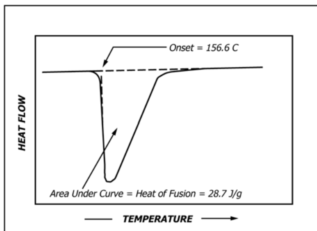
FIG. 1 Indium Calibration
