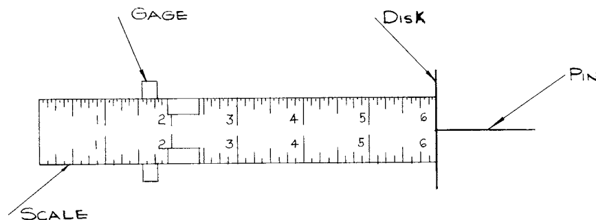
FIG. 1 Thickness Gage
