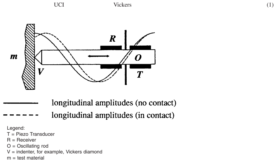
FIG. 1 Schematic Description of the UCI Probe
