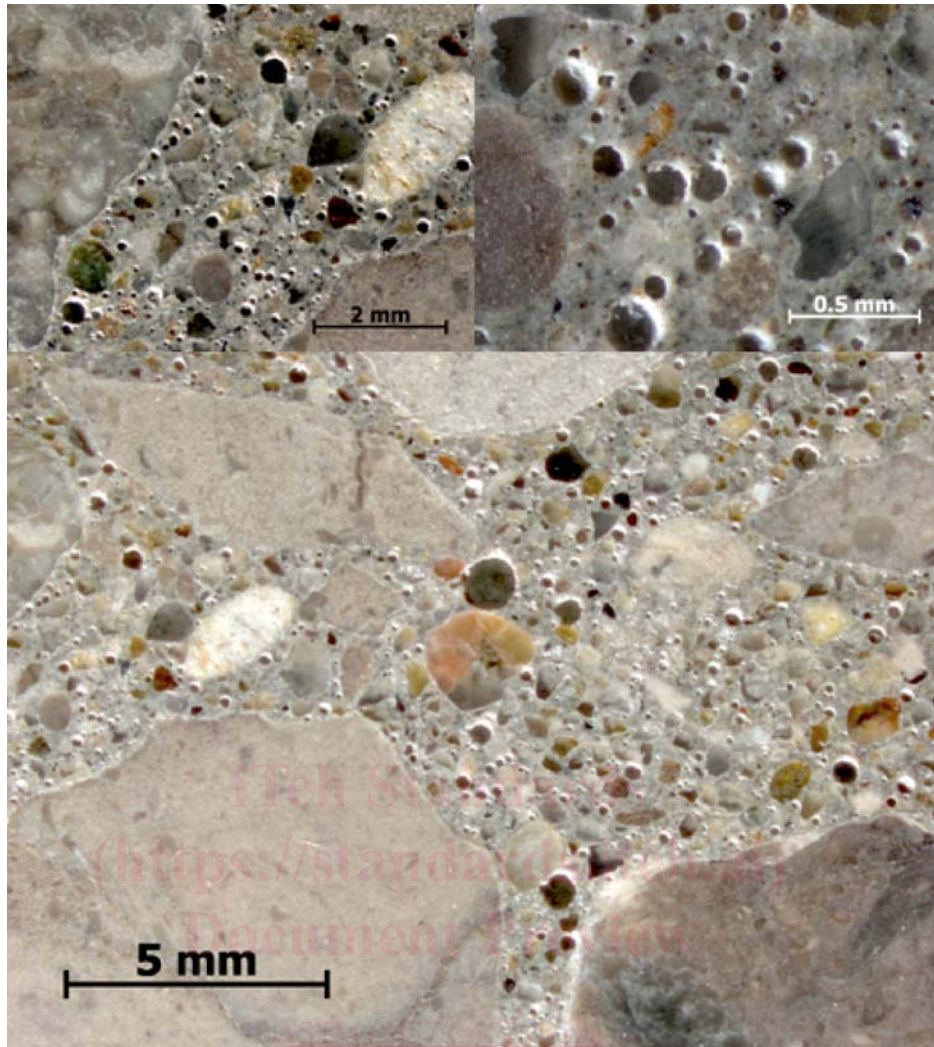
https://standards.iteh.ai/catalog/standards/7738a4db/astm-c457-c457m-10a FIG. 1 Photographs of a Satisfactory Surface
