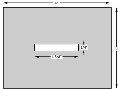
FIG. 3 Mask I Containing a Slot Just Smaller Than the Blue Wool References
