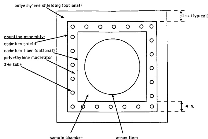
FIG.-2 1 A Cross-section View of a Typical Thermal-Neutron Coincidence Counter
