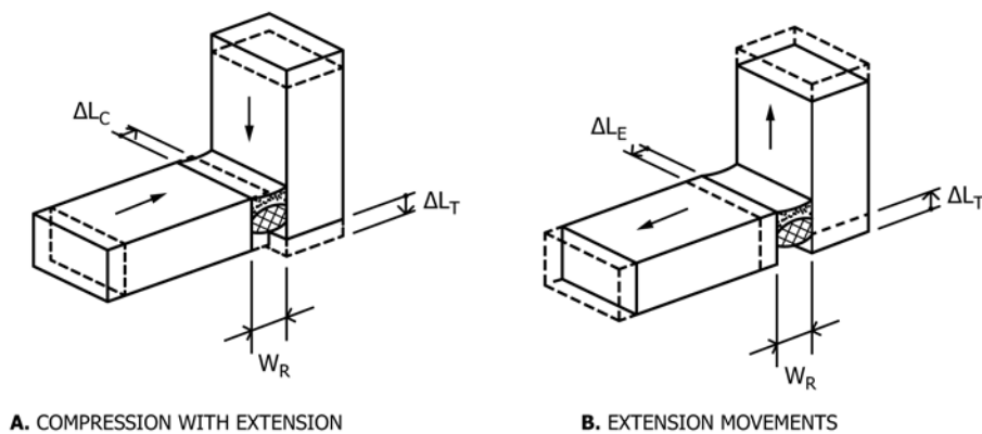
FIG. 3 Extension and Compression Movement with Transverse Extension
