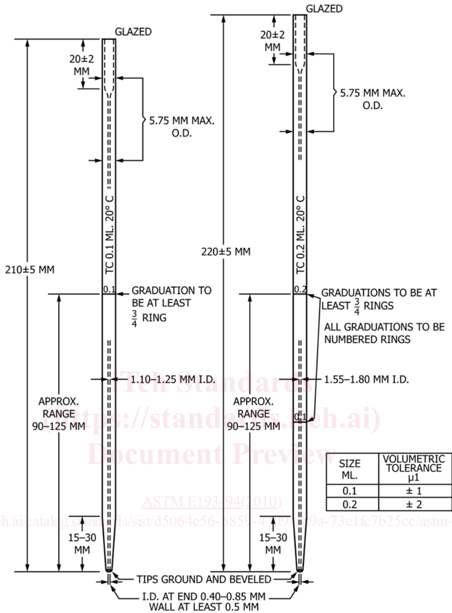
FIG. 2 Micropipets, Folin-Type
