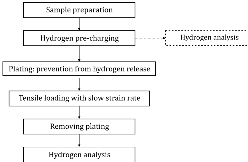
Figure 1 — Flow chart illustrating the test methods
