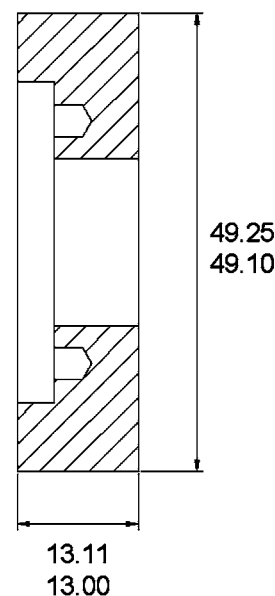
FIG. 1 Ball-on-Cylinder Test Ring
