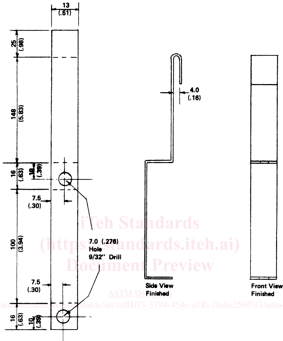
FIG. 3 Thermometer Bracket
