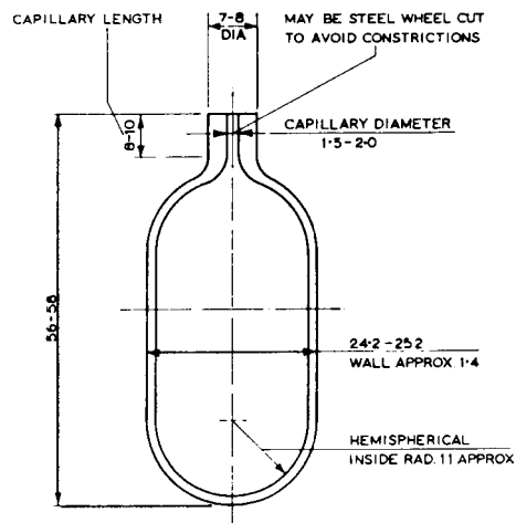
NOTE—All dimensions are in millimetres. FIG. 1 Glass Coking Bulb
