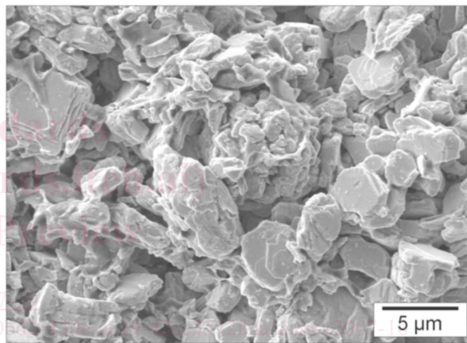
Illustration courtesy of Carestream Health FIG. 9 Conventional BaFX: Eu Grains (5 microns)
