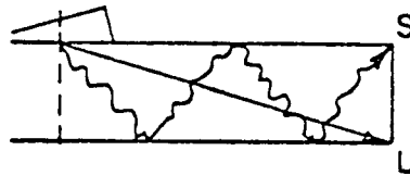
FIG. 7 Coincident Beams
