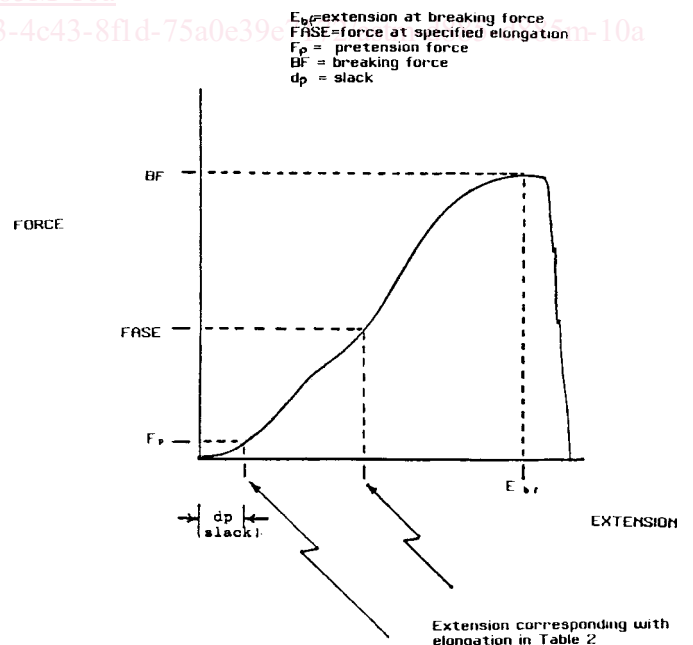
FIG. 1 Force-Extension Curve
