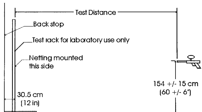
FIG. 1 Testing Apparatus Layout
