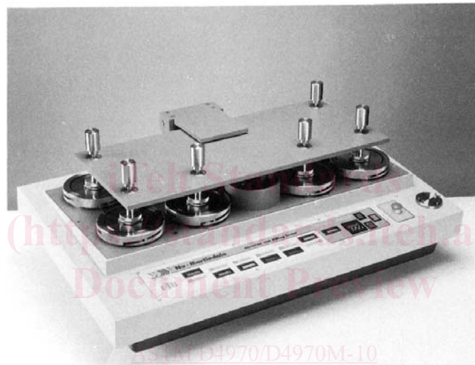
FIG. 1 Martindale Abrasion Tester
