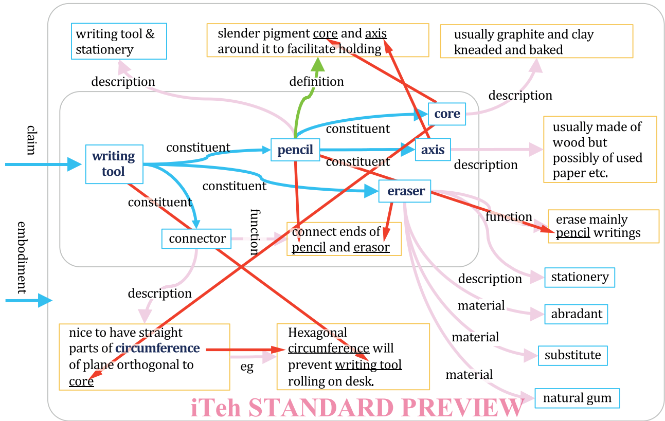
Figure A.2 — Anaphoric links in graph segment
