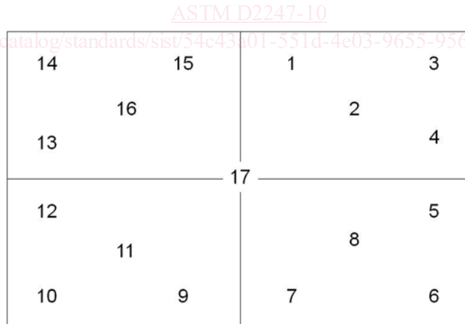
FIG. A1.1 Diagram of Specimen Placement for Mapping Chamber for Condensation Uniformity
