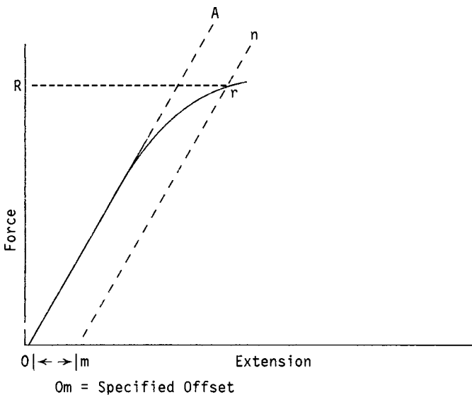
FIG. 1 Force-Extension Curve for Determination of Yield Strength by the Offset Method
