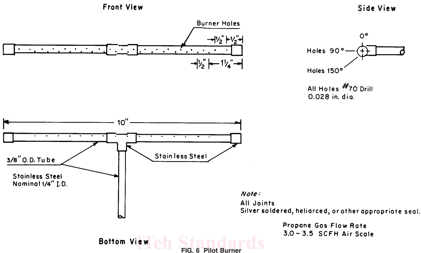
FIG. 6 Pilot Burner
