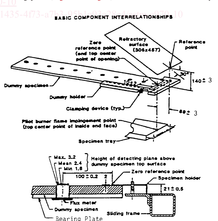
FIG. 3 Zero Reference Point Related to Detecting Plane
