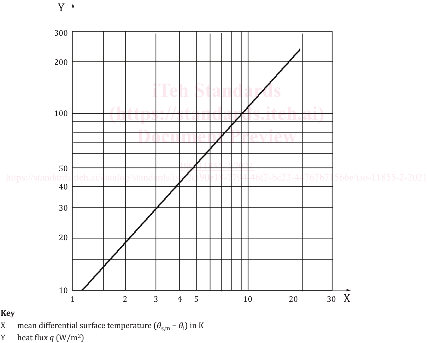
Figure 1 — Basic characteristic curve for floor heating and ceiling cooling
