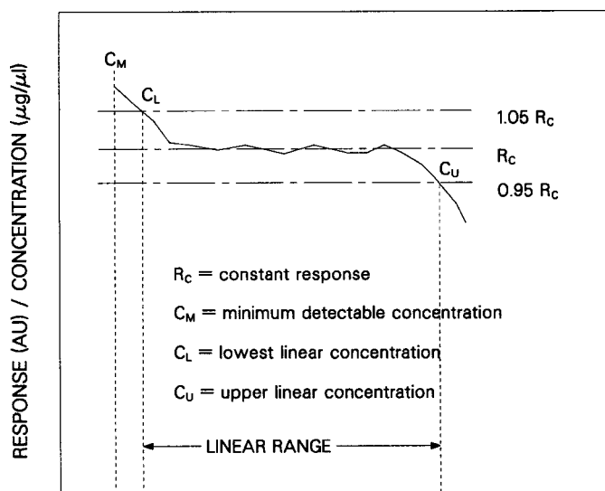
FIG. 1 Example of a Linearity Plot for a Photometric Detector
