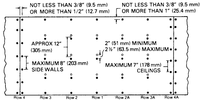
FIG. 1 Double Nailing
