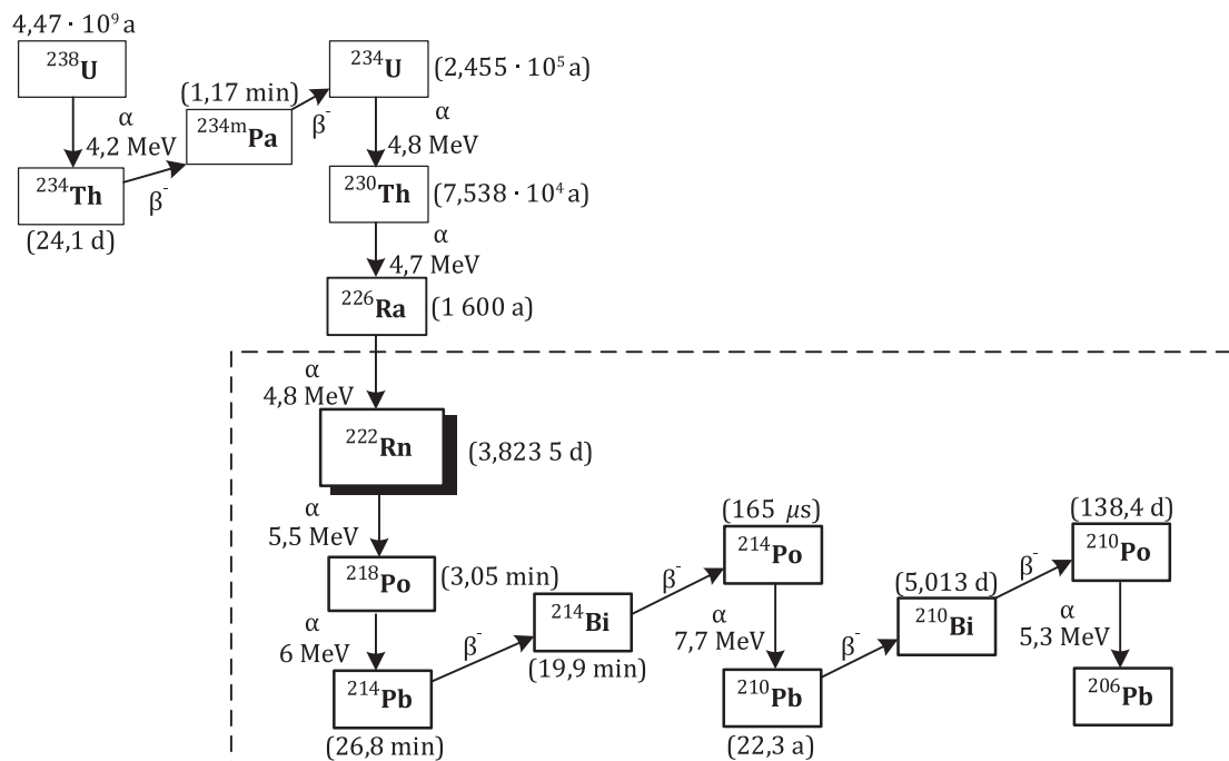
Figure 1 – Uranium-238 and its decay products (standards.iteh.ai)
