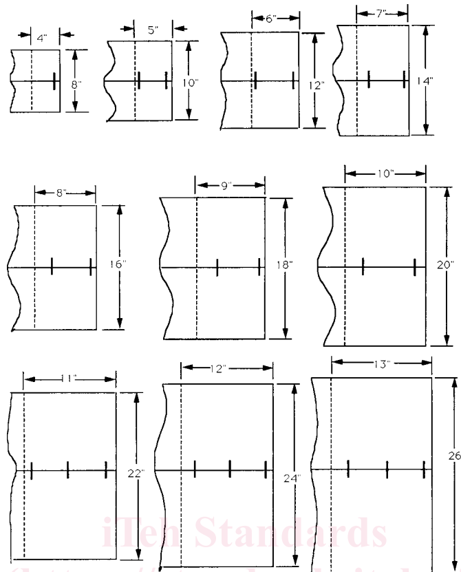
FIG.-8 9 Example of Closure Method 2D4
