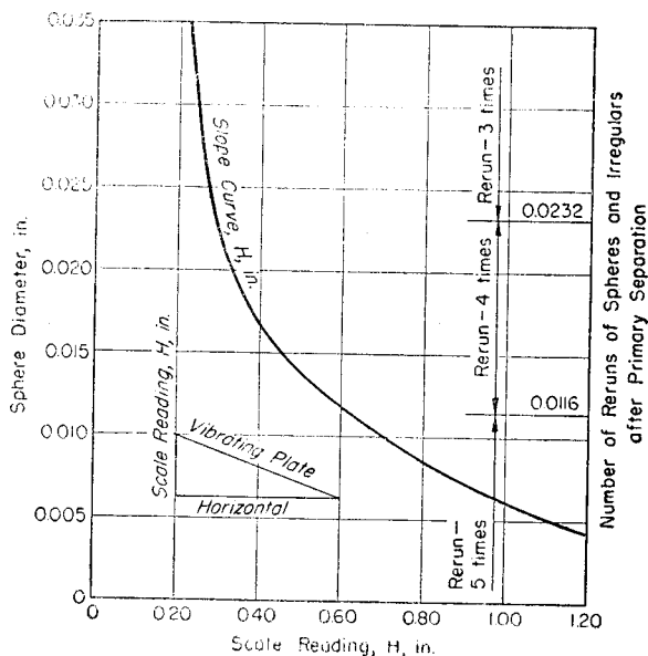
FIG. 2 Angle Calibration Curve for Setting the Roundness Tester Inclination with a Digital Level
