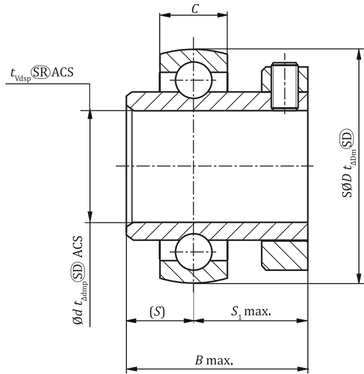
Figure 2 — Bearing with concentric locking collars around the inner ring — Intermediate overall width
