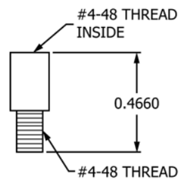
FIG. 3 Contact Extension
