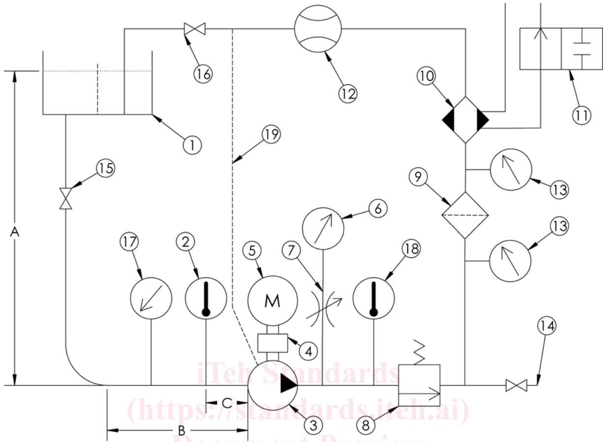
FIG. 1 System Schematic
