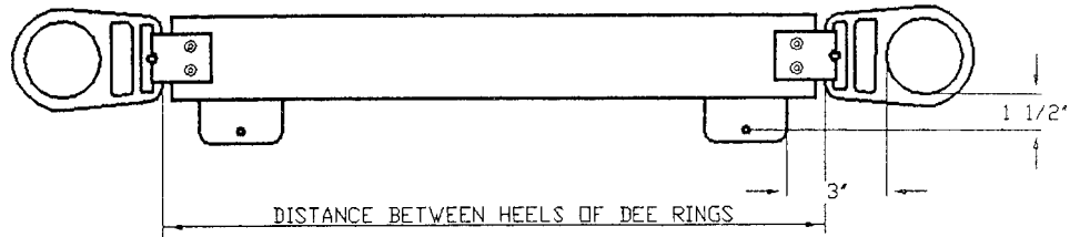
FIG. 10 "Dee" Measurement
