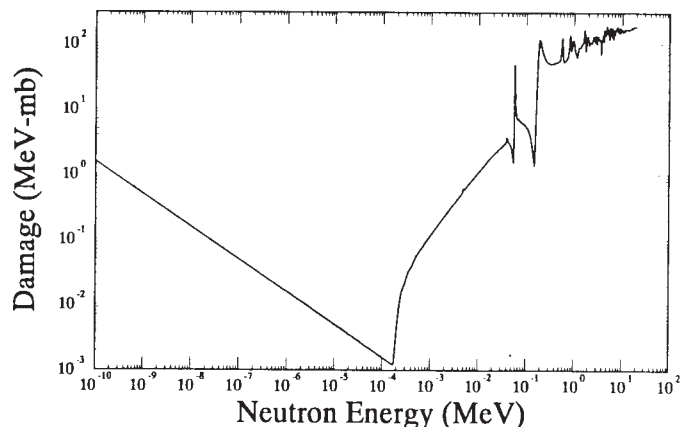
FIG. A1.1 Silicon Damage Function
