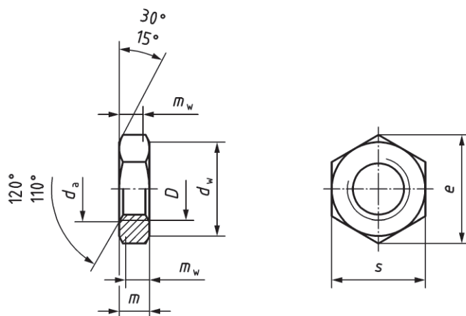
Figure 1 — Nuts without washer-face (standards.iteh.ai)
