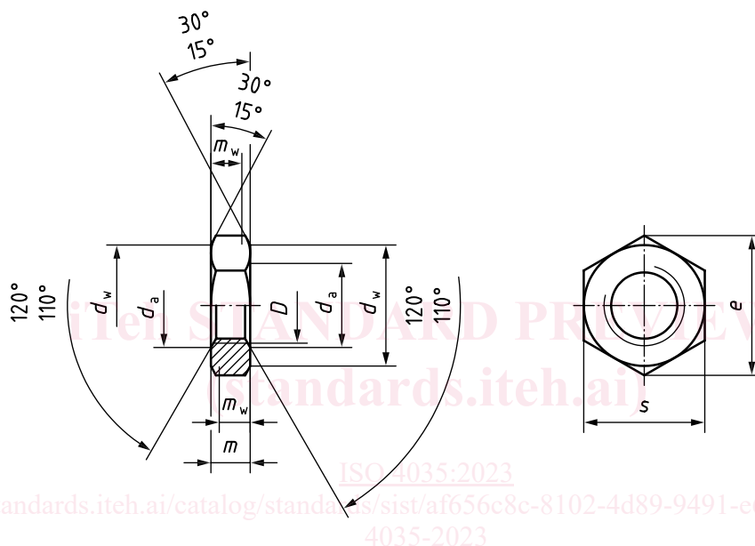
Figure 1 — Ecrou bas hexagonal
