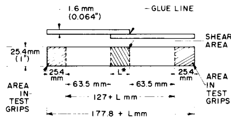
FIG. 1 Form and Dimensions of Test Specimen
