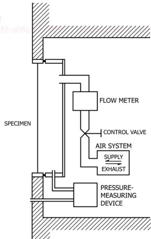
FIG. 1 General Arrangement of Air Leakage Test Apparatus
