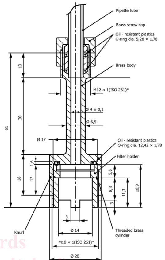
FIG. 7 Filter Unit
