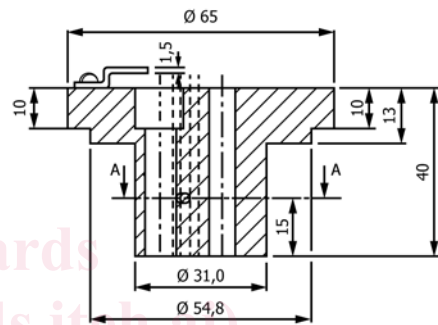
FIG. 4 Supporting Ring
