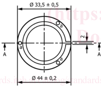
FIG. 2 Watertight Brass Jacket
