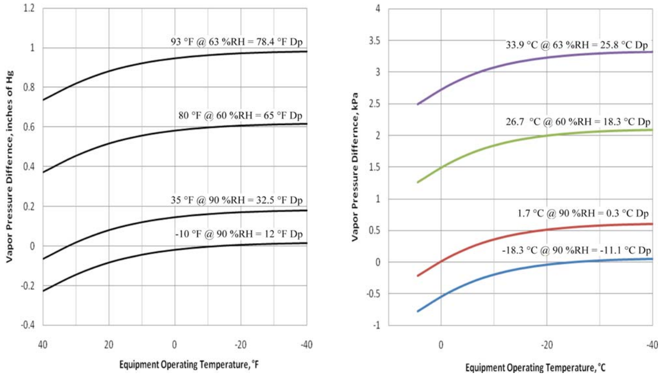
FIG. 2 Magnitude of Water Vapor Pressure Difference for Selected Conditions (Derived from Fig. 1)
