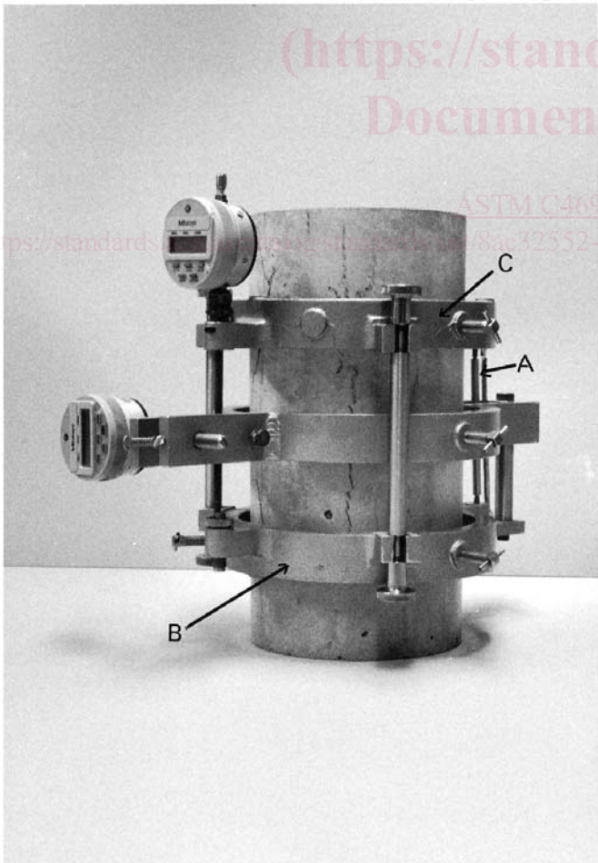
FIG. 1 Suitable Compressometer
