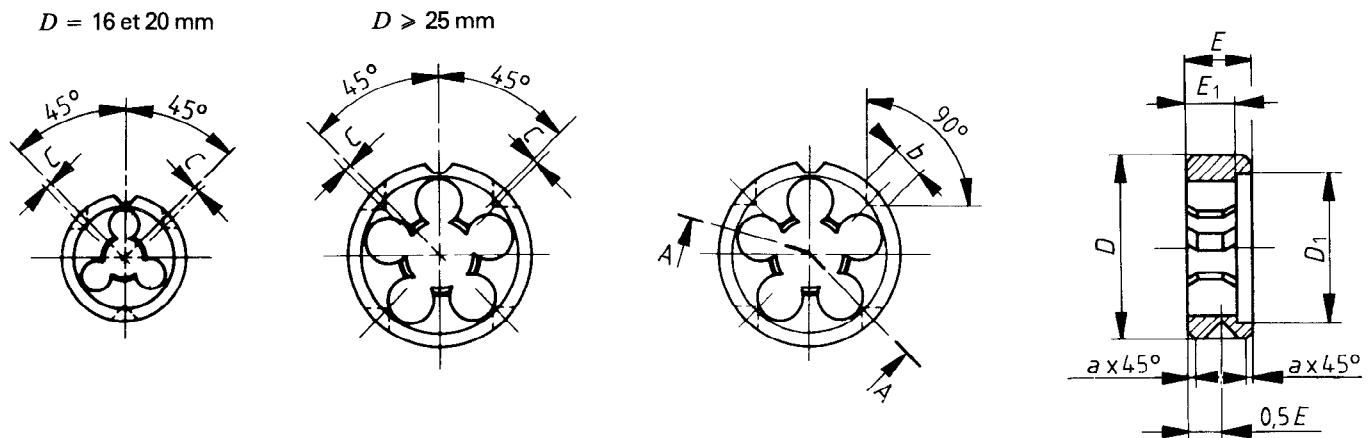
Figure 2 — Filières UNC et UNF
