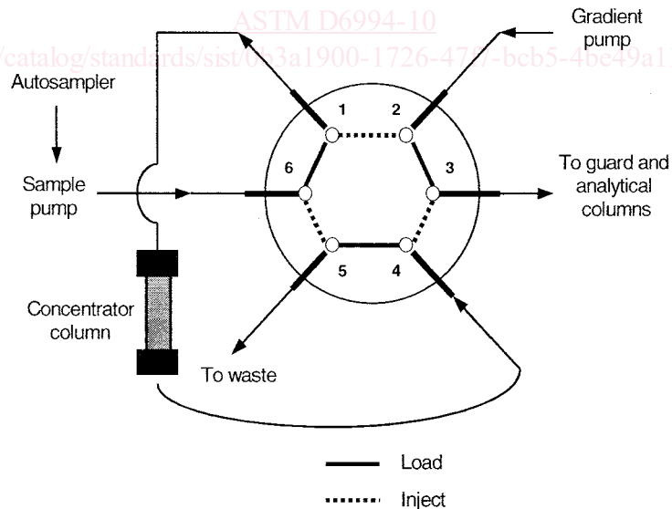
FIG. 5 Injection Valve Configuration for Sample Preconcentration
