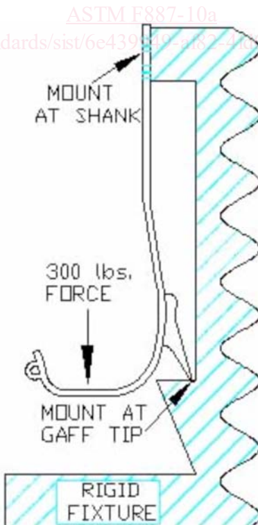
FIG. 5 Fatigue Test Fixture
