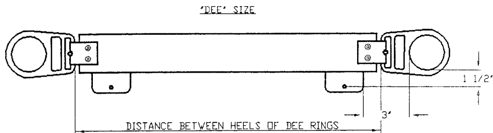
FIG. 10 “Dee” Measurement
