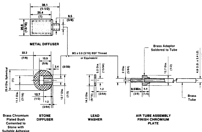
FIG. 2 Attachment of Gas Diffusers to Air-Inlet Tubes
