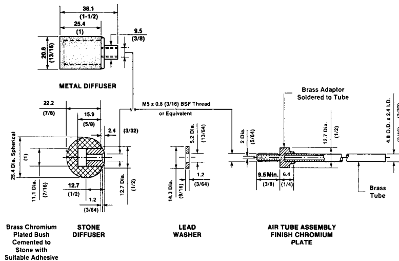
Dimensions in millimetres (inches) FIG. 2 Attachment of Gas Diffusers to Air-Inlet Tubes
