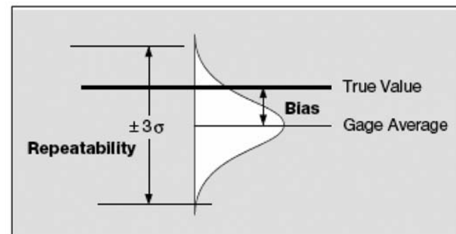
FIG. 1 Repeatability and Bias Concepts
