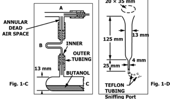
FIG. X1.1 Butanol Scale Olfactometer
