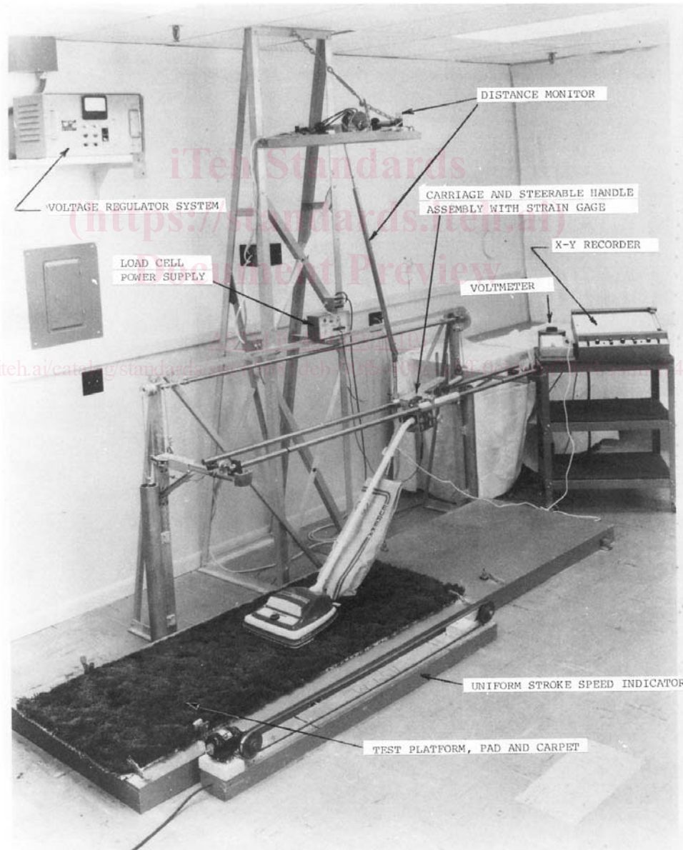
FIG. 1 ASTM Mobility Fixture and Associated Equipment
