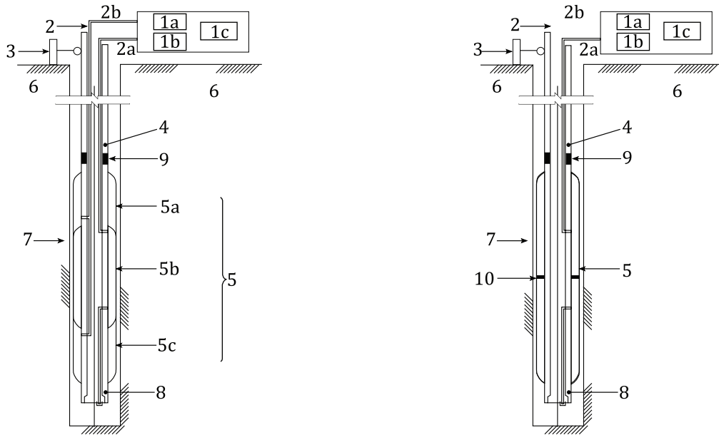
a) Thi-cell probes, E type, with measurement of volume of the measuring cell
