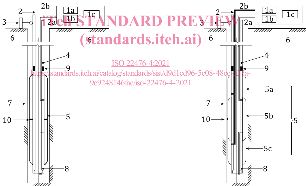
c) Mono-cell probe, with measurement of radial displacement (optional)
