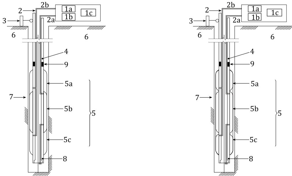
a) Tri-cell probe, G type, with measurement of volume of the measuring cell
